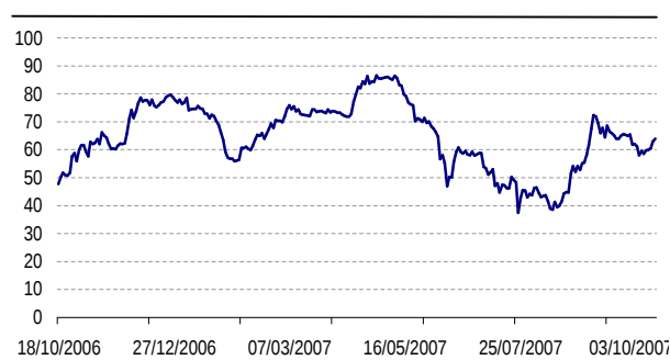
Bank of Moscow15 vs VTB15 spread
