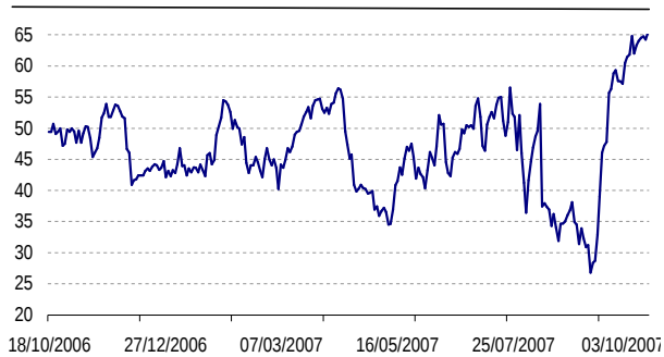
Gazprom20 vs Gazprom13 spread
